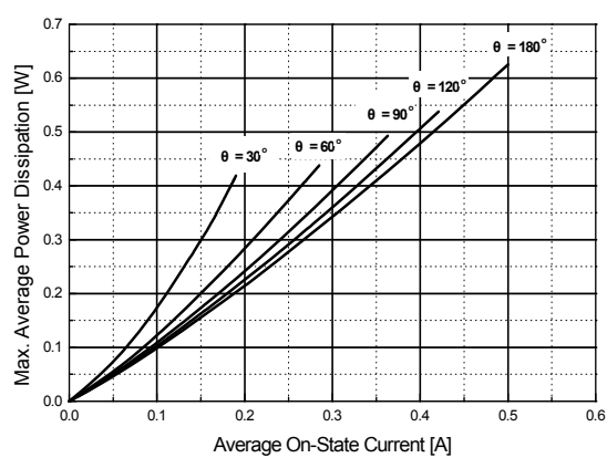
Fig 8. Power Dissipation
